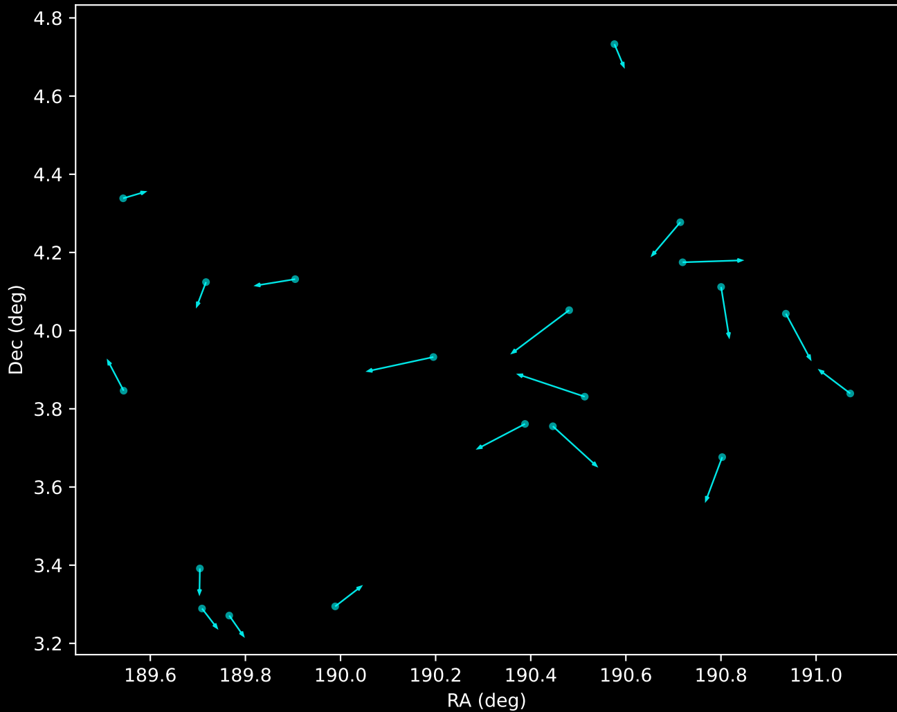
GALAH DR4 Noise Stream Proper Motion Vectors (n=20)
