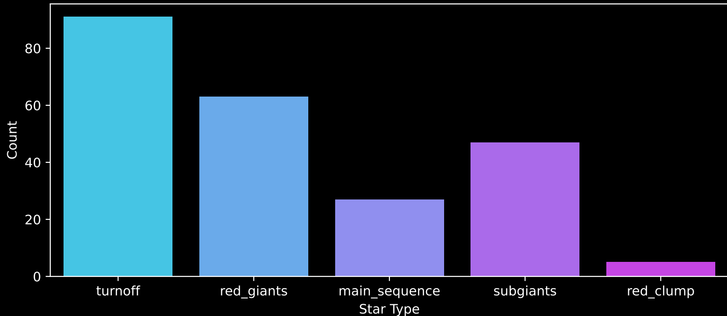
GALAH DR4 Field: [9332] Count plot of Star Type
