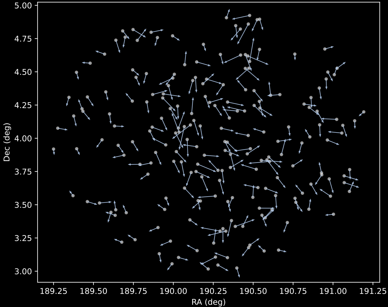
GALAH DR4 Cluster 1 Proper Motion Vectors (n=208)
