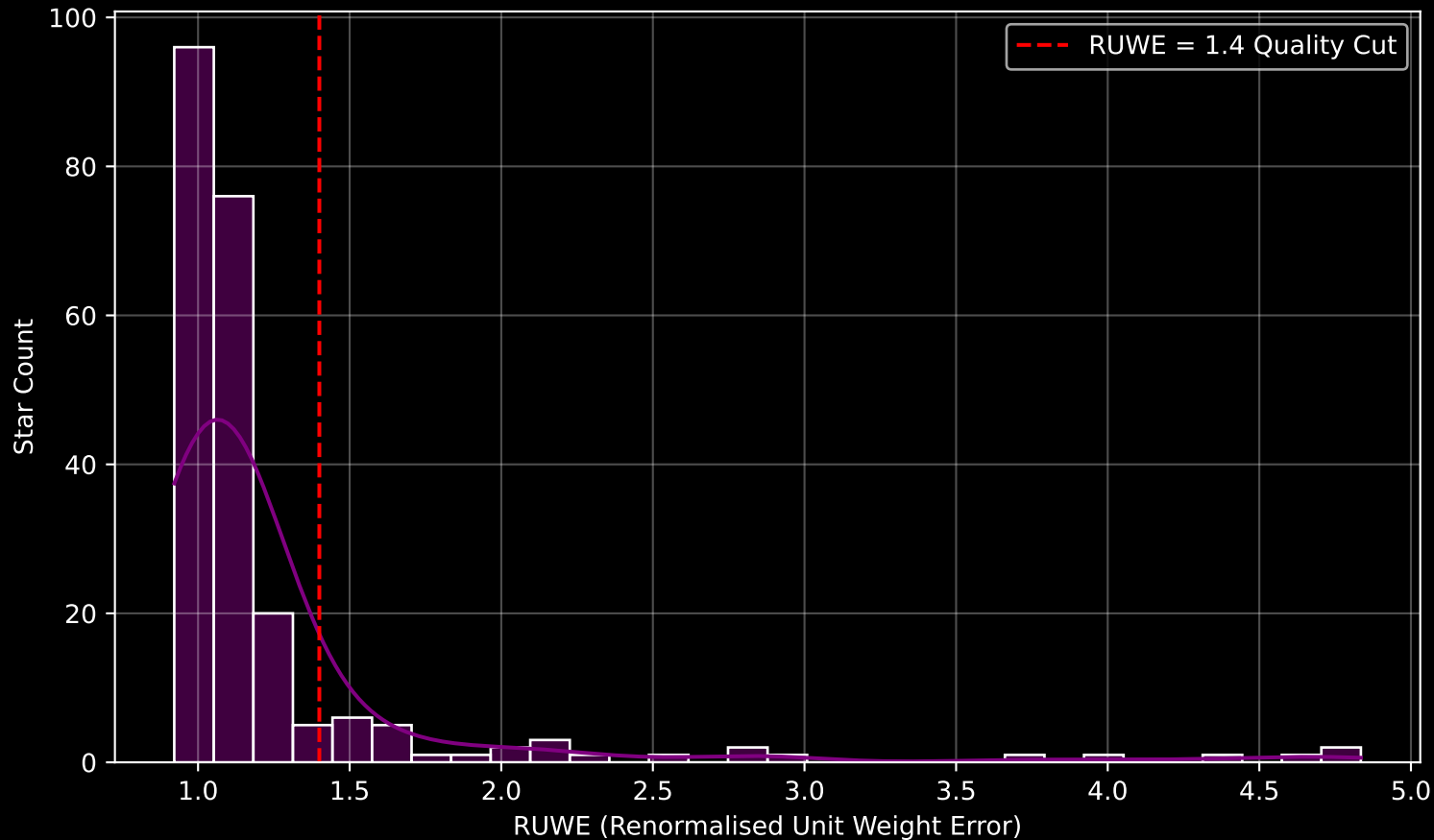
GALAH DR4 Field [9332] RUWE Distribution (n= 226)
